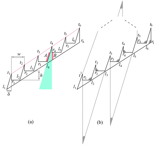
Figure 1: (a) Polygon P construction. (b) Localizing P with n/2 general guards.
