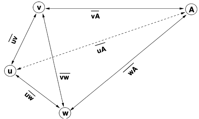
Fig. 32. Upon receiving distances \overline{vA} and \overline{wA} from v and w , node u estimates its distances to v ( \overline{uv} ) and w ( \overline{uw} ) and uses trigonometry to estimate its distance to A ( \overline{uA} ).
