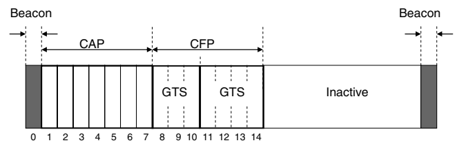
Fig. 1. MAC super-frame.
