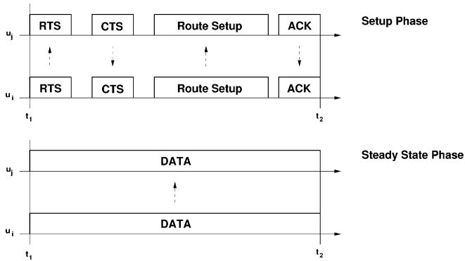
Fig. 17. Flexible stream scheduling phases: In the Setup Phase node u_i , reserves time interval [t_1, t_2] with a RTS/CTS/RouteSetup/ACK protocol exchange for communication to u_j ; In the Steady State Phase u_i , uses intervals [t_1, t_2] to send data packets to u_j .
