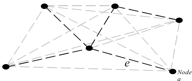
Fig. 19. Euclidean minimum spanning tree.
