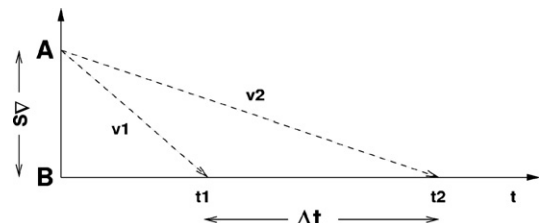
Fig. 29. TDoA principles: A sends B two messages propagating with speeds v_1 and v_2 and arriving at times t_1 and t_2 . Knowing v_1 and v_2 and measuring \Delta t = t_2 - t_1 , B can estimate the distance to A as \Delta s = \frac{v_1 \cdot v_2}{v_1 - v_2} \cdot \Delta t .
