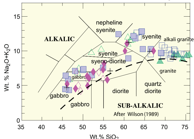
Figure 4. Nomenclature of plutonic rocks after Wilson (1989). The heavy dashed line separates alkalic and sub-alkalic rocks. Data symbols are the same as in Figure 3.
