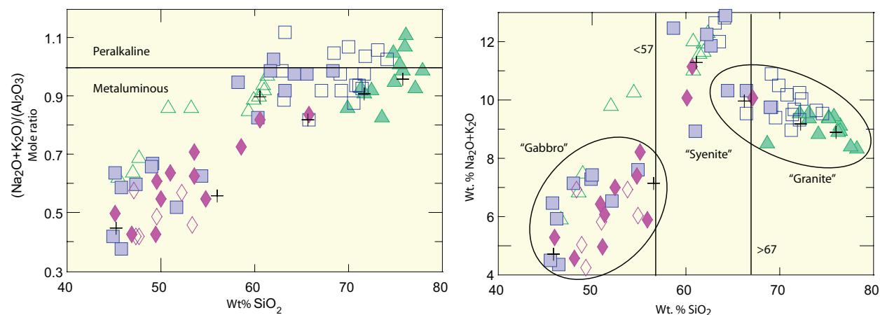
Figure 6. Aluminum saturation classification showing the mole ratio (Na_2O + K_2O)/(Al_2O_3) plotted against weight percent silica. Although all mafic, low silica rocks have normal alumina contents, some of the higher silica granites are peralkaline. Data symbols are the same as in Figure 3.
