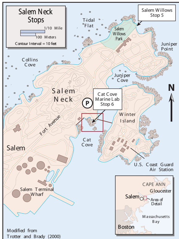
Figure 19. On the left is a location map for the Salem Neck stops. On the right is a photomicrograph of the trachytic syenite from Salem Willows Park viewed in cross-polarized light.
