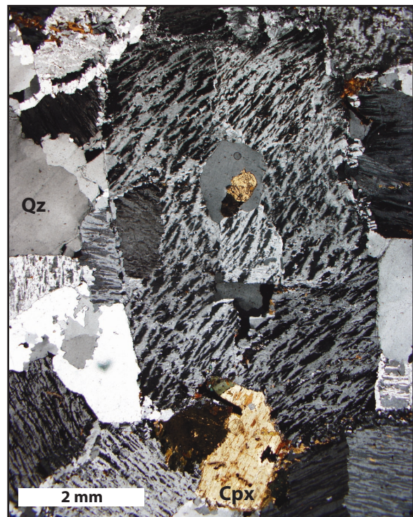
Figure 14. A photomicrograph of the Cape Ann granite in crossed-polarized light showing the microperthite texture. Quartz (Qz) and aegirine-augite (Cpx) are also visible.
