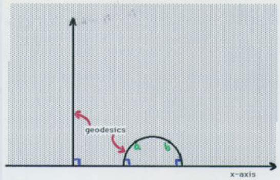
Hyperbolic 2-Space The Upper Half Plane Model H^2 = \{(x,y): y>0\}
