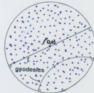
Hyperbolic 2-Space
