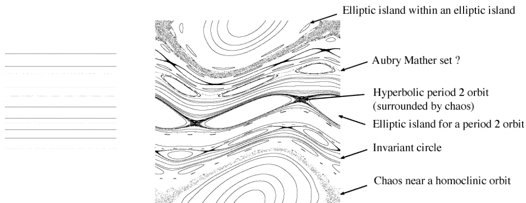
Fig. 1.1. The different dynamics in the standard map: the left hand side shows a selection of orbits for the completely integrable F_0 , all on invariant circles. The right hand side displays orbits for F_\epsilon with \epsilon = .817 .
