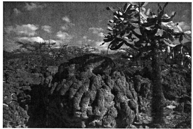
Figure 7. Large serpulid-tufa mound located along the northern shore of Lago Enriquillo. Mound is approximately 2 m in height; intervals on Jacob's staff = 10 cm.
