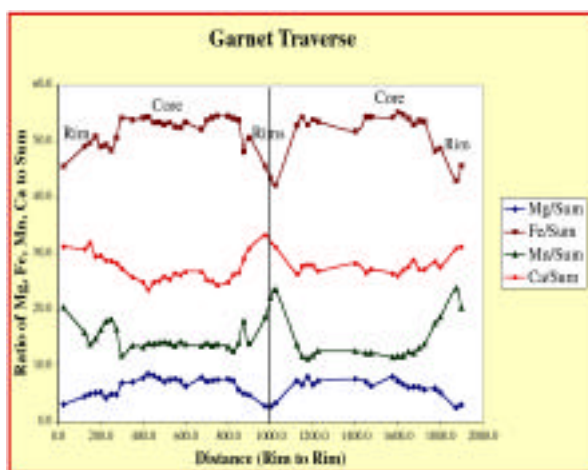
Figure 6. Garnets have higher Mg and Fe in the cores.
