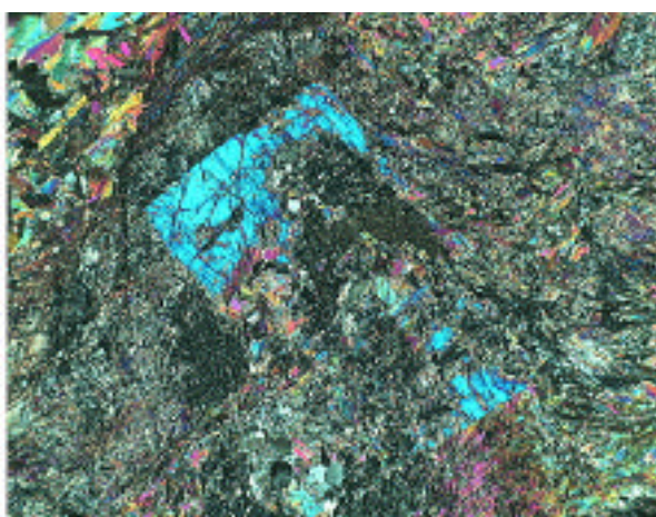
Figure 3. Pseudomorph with remnant lawsonite (crossed polars)
