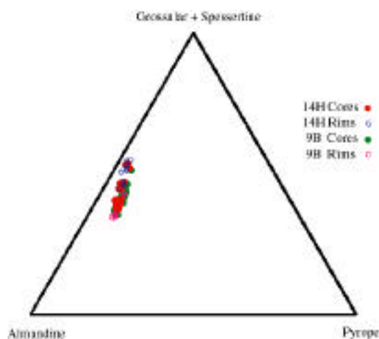
Figure 5. Garnet has little pyrope.
