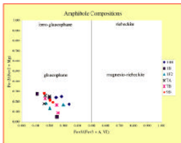
Figure 4. Na-Amphiboles plot in glaucophane quadrant.
