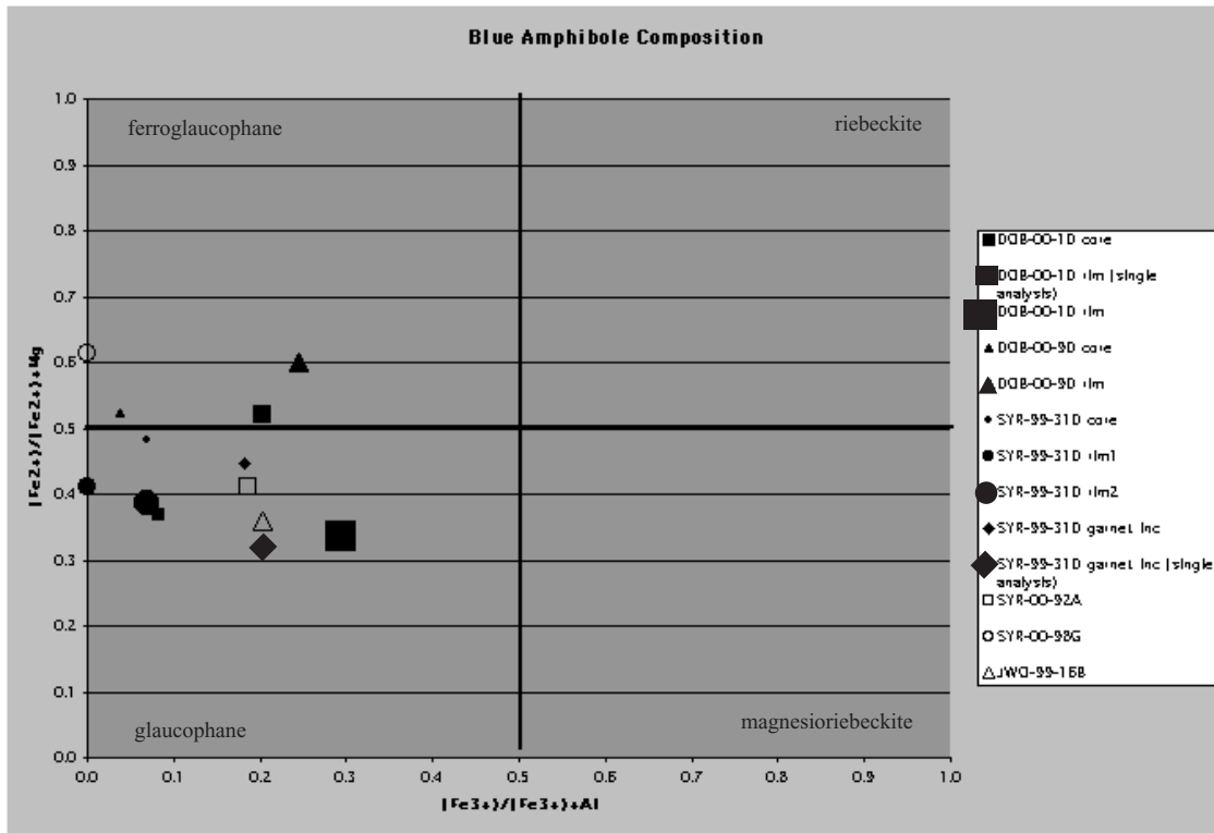
Figure 3. Composition of blue amphiboles. Amphiboles were corrected for ferric iron using several stoichiometric assumptions, including \text{Si}=8 for a lower bound and \bullet\text{Mg}=13 and \bullet\text{Na}=15 for upper bounds. The greatest lower bound and least upper bound that yielded reasonable stoichiometries were averaged to obtain an estimated composition. Zoned amphiboles occur in some samples and are characterized by compositions of rims vs. cores. Included in the chart are single analyses that have good weight percent totals, but are noticeably different from the averages.
