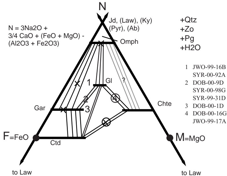
Figure 1. NFM Projection from quartz, zoisite and paragonite onto the plane \text{NaAlO}_2\text{-FeAl}_2\text{O}_4\text{-MgAl}_2\text{O}_4 . Phases are plotted schematically. Xs and numbers mark approximate bulk compositions as estimated from assemblages seen in thin section. Numbers refer to samples analyzed using the SEM/EDS and circled symbols are + garnet. Chlorite-omphacite may not be stable with these other assemblages.
