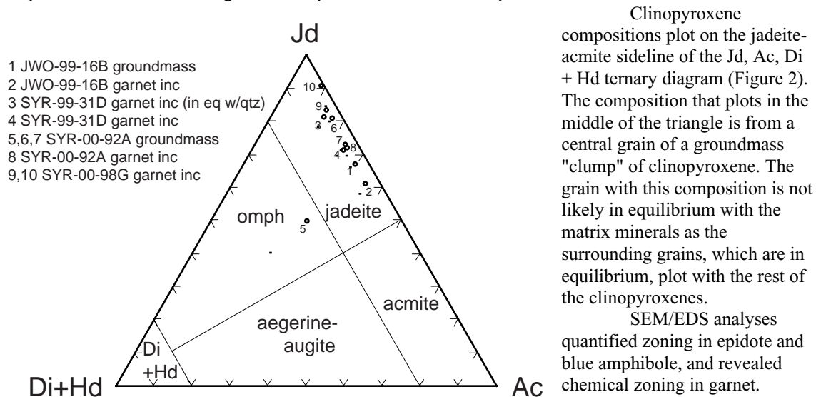
Figure 2. Averaged Clinopyroxene composition. Most pyroxenes plot along the jadeite-acmite sideline within the jadeite zone of this triangle. The omphacite is not likely in equilibrium with the matrix minerals.
