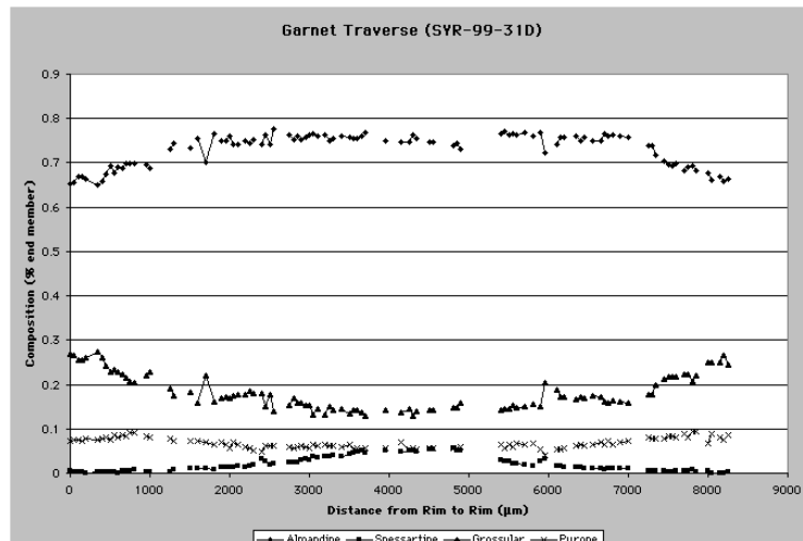
Figure 4. Traverse across a garnet from SYR-99-31D quantifying undulatory zoning. Notice that unlike the analyses of the majority of garnets studied, this traverse shows almost perfectly defined calcium-iron and manganese-magnesium substitutions.
