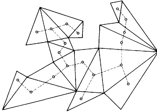
Fig. 1.14. The dual of a polygon triangulation is a tree.
