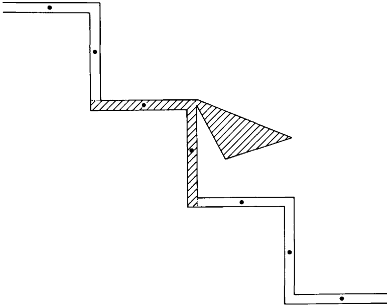
Fig. 9.7. The triangular region is covered free when the truth assignment covers the shaded distinguished points.
