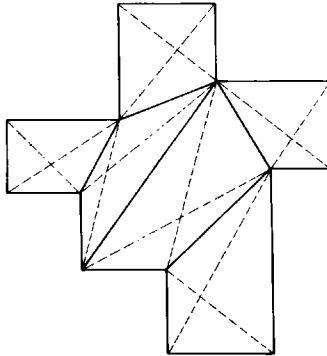
Fig. 2.19. A 4-colorable graph derived from a quadrilateralization by adding all quadrilateral diagonals.
