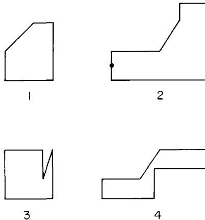
Fig. 2.29. Four unquadrilateralizable polygons, each violating one of the 1-orthogonal conditions.
