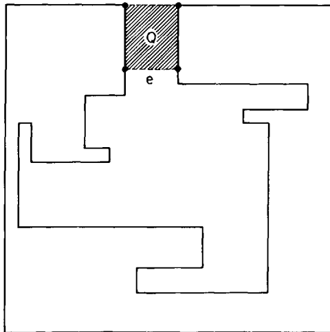
Fig. 6.5. The exterior of an orthogonal polygon may be converted into the interior of another by deleting the highest edge e and enclosing within a rectangle.
