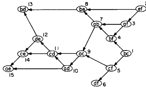
Fig. 8.11. The directed graph associated with the arrangement in Fig. 8.9, and a topological sort.
