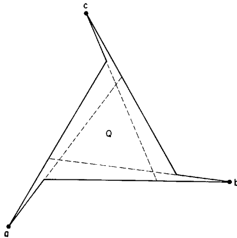
Fig. 1.4. Guards at a , b , and c cover the boundary but not the interior of the polygon.
