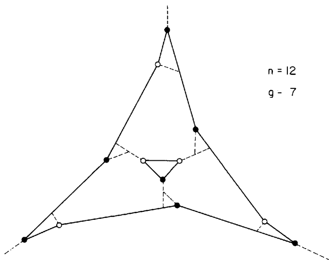
Fig. 6.19. A convex partitioning of 12 vertices that requires 7 combinatorial guards (solid dots) for domination.
