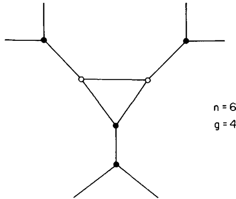
Fig. 6.18. A convex partitioning of 6 vertices that requires 4 combinatorial guards (solid dots) for domination.
