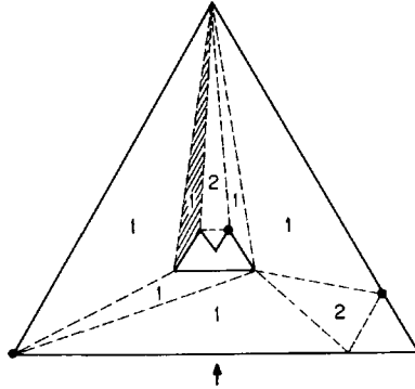
Fig. 5.8. A triangulation of 10 vertices with string 121/121/1/1/ that requires 4 guards: the 3 shown (dots) do not cover the shaded triangle.
