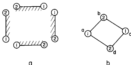
Fig. 2.36. Vertex types; the shading in (a) represents the polygon interior.
