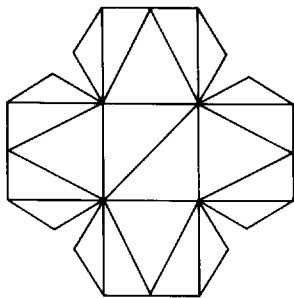
Fig. 1.8. No diagonal of this triangulation cuts off exactly three vertices.
