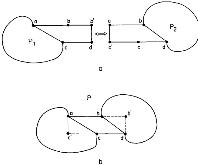
Fig. 2.8. Reduction for non-tab neighboring edges ab and cd .
