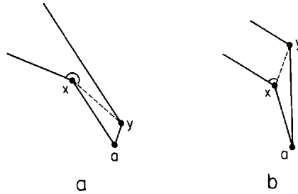
Fig. 4.10. Cutting off an ear from a spiral.
