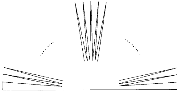
Fig. 4.2. A star polygon that requires \lfloor r/2 \rfloor + 1 vertex guards.
