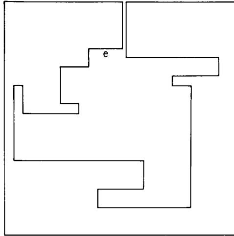
Fig. 6.6. An alternative enclosing strategy, used when n is divisible by 4.
