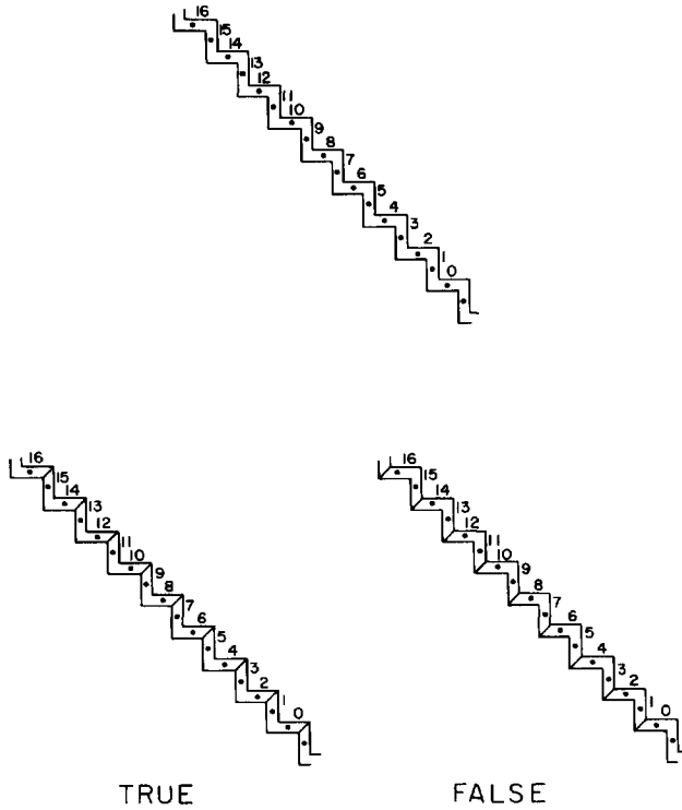
Fig. 9.4. The truth-setting component has two distinct minimum covers corresponding to assignments true and false .
