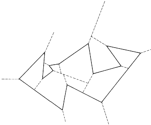
Fig. 6.17. A convex partitioning of the plane induced by a polygon; here n = 14 and 15 regions result.
