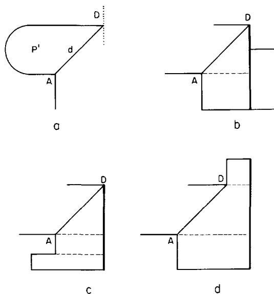
Fig. 3.34. When the edges adjacent to d have the same parity, Lemma 3.21 applies in all cases.
