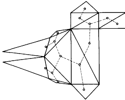
Fig. 1.20. The triangulation dual of a monotone polygon is not necessarily a path.
