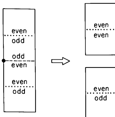
Fig. 2.57. Partitioning at an odd-cut can either flip or leave the parity of other cuts unchanged when the total number of reflex vertices is even.
