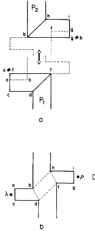
Fig. 2.13. Tab pair reduction.
