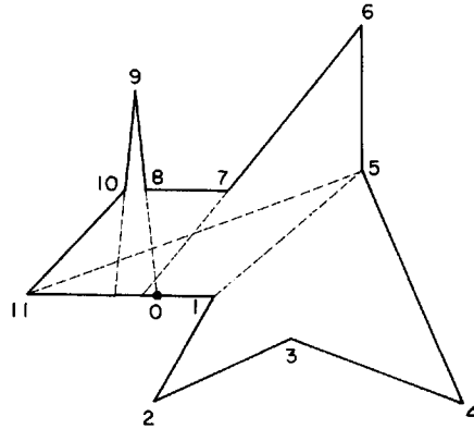
Fig. 9.22. An example of the star partitioning algorithm: the polygon may be partitioned into two stars.
