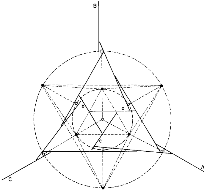
Fig. 10.8. A pattern of 12 line segments that require 7 point guards.
