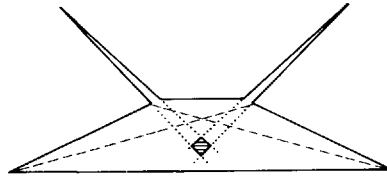
Fig. 4.5. No diagonal intersects the kernel (shaded).
