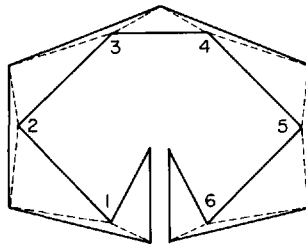
Fig. 4.11. A spiral polygon requiring \lfloor (n + 2)/5 \rfloor diagonal guards.
