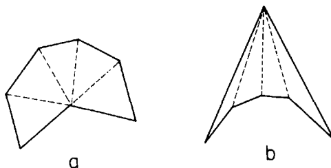
Fig. 4.9. Path triangulations of spiral polygons with one reflex vertex (a) and three convex vertices (b).
