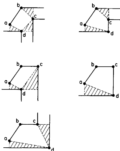
Fig. 2.35. The noses of the diagonals of the removable quadrilateral are all empty (shaded regions).
