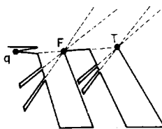
Fig. 9.12. A variable pattern. The distinguished point q can be seen only by T and F .
