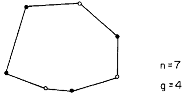
Fig. 6.1. A convex polygon requires \lceil n/2 \rceil vertex guards (solid dots) to cover the exterior.
