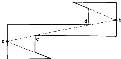
Fig. 9.3. A polygon that can be covered with 2 stars if diagonal cd is used, but that requires 3 if only edge extensions are used.
