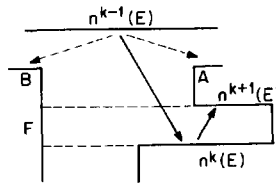
Fig. 2.15. E falls between F and the top edge of tab(E) .
