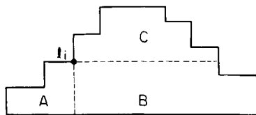
Fig. 2.21. l_i is connected to a vertex in B .
