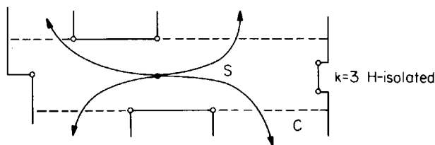
Fig. 2.51. A source region S admits an H-odd-cut if it contains k \neq 1 H-isolated vertices.
