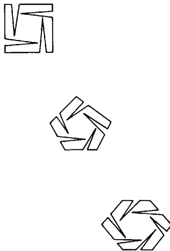
Fig. 1.27. “Shutter” shapes show that r guards can be necessary.
