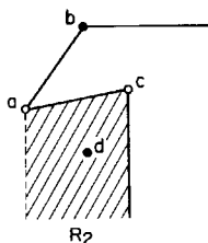
Fig. 2.33. Definition of vertex d and region R_2 .
