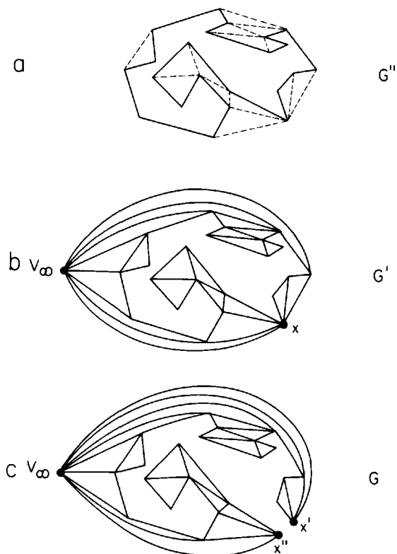
Fig. 6.3. The graph G in (c) is produced from a triangulation of the hull pockets (a) by connecting all hull vertices to v_\infty (b) and splitting some hull vertex x .
