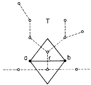
Fig. 5.5. A tree T attached at diagonal ab to a cycle, which extends to the left and right.
