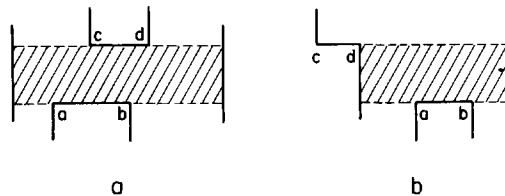
Fig. 2.25. Empty rectangles above bottom peaks.
