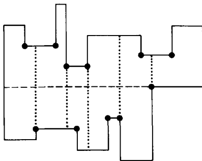
Fig. 2.59. Polygons with no horizontal odd-cuts have a horizontal cut (dashed) that partitions them into two vertical histograms, which can then be cut vertically into L-shaped pieces at every other reflex vertex.
