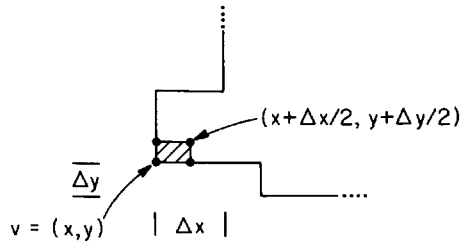
Fig. 2.53. A reflex vertex introduced by removing a “chip” from the polygon at a convex vertex v .
