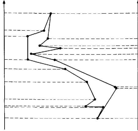
Fig. 1.15. The vertices of a monotone polygon project onto a line in a monotonically increasing sequence.
