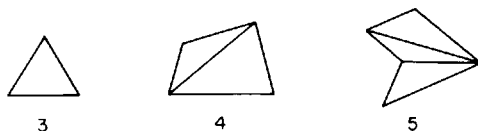
Fig. 1.7. Triangulations of up to five vertices are necessarily fans.
