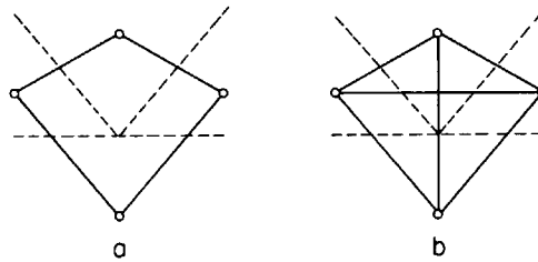
Fig. 10.7. If three segments (dashed) meet at a point, either dual graph is not a triangulation (a) or it is not necessarily planar (b).
