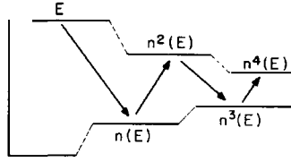
Fig. 2.14. The chain induced by n(E) leads to tab(E) .
