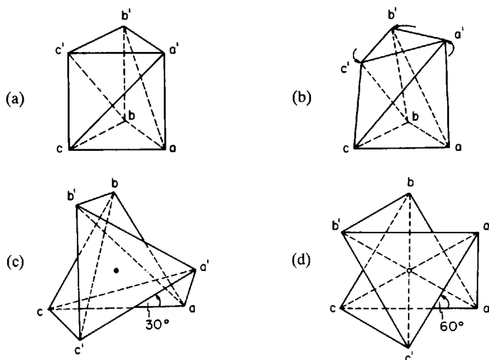
Fig. 10.1. Schönhardt's untetrahedralizable polyhedron, constructed by twisting the top of a triangular prism (a) by 30^\circ , producing (b), shown in top view (c); a twist of 60^\circ would cause face intersections (d).
