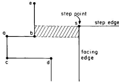
Fig. 2.9. Definitions of tab components; the tab (ab, cd) is bad.
