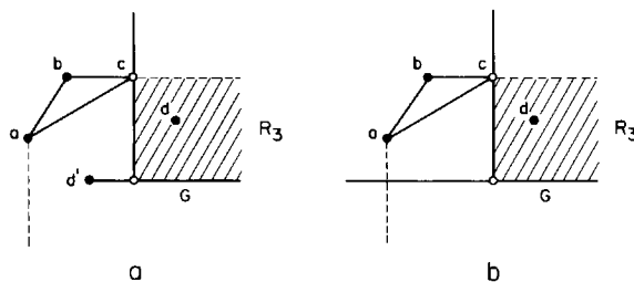
Fig. 2.34. Definition of vertex d and region R_3 .
