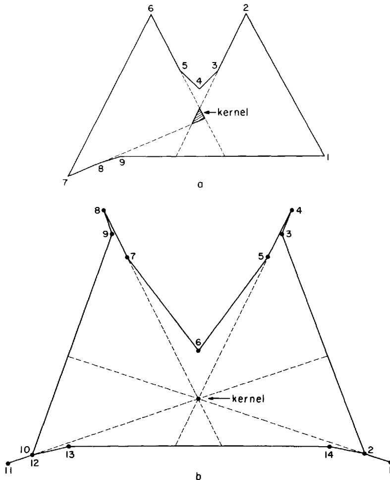
Fig. 4.6. Two star polygons that each require two diagonal guards, due to Shermer (a) and Suri (b).
