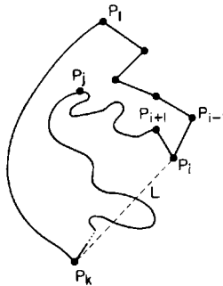
Fig. 1.16. If p_i is not an interior cusp, then p_j is.
