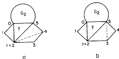
Fig. 1.10. G_1 is a hexagon.
