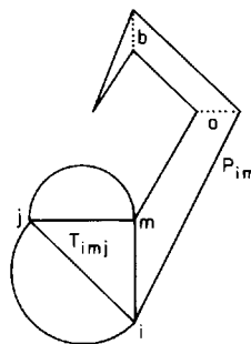
Fig. 9.19. T_{imj} cannot merge with every minimal partition of P_{im} .
