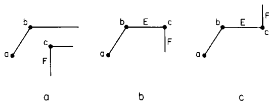
Fig. 2.32. Either c is at a corner (a) or at the other end of E (b and c).
