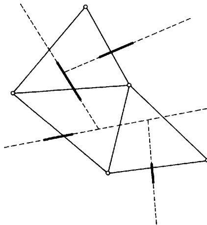
Fig. 10.6. A convex partition of the plane induced by a set of line segments (shown bold) and its dual graph.
