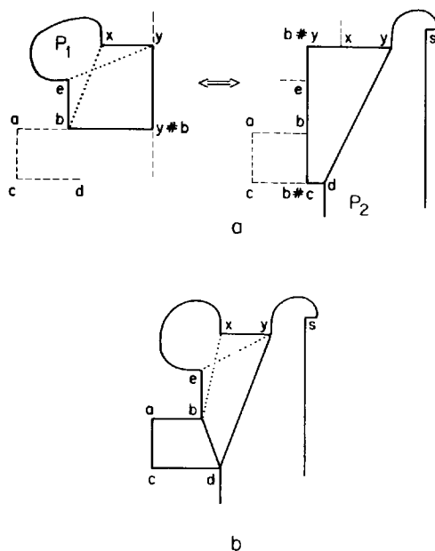
Fig. 2.12. Good tab reduction for Fig. 2.10b.
