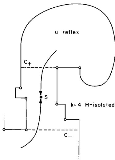
Fig. 2.49. A sink region S always permits an odd-cut.
