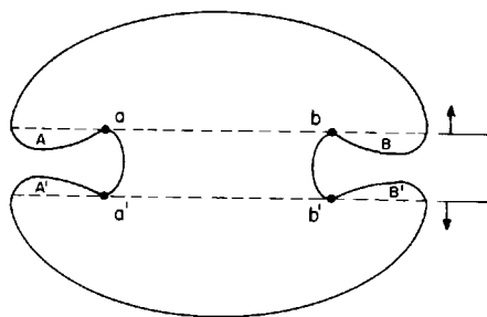
Fig. 10.14. A region not illuminable from any one point.
