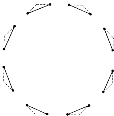
Fig. 10.10. An arrangement of 8 line segments that require 8 vertex guards.
