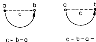
Fig. 2.56. The labels a and b assigned to the two ends of a cut determine the number of reflex vertices c to one side by their difference or difference less 1.
