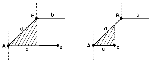
Fig. 3.23. The partial shadow of a diagonal.
