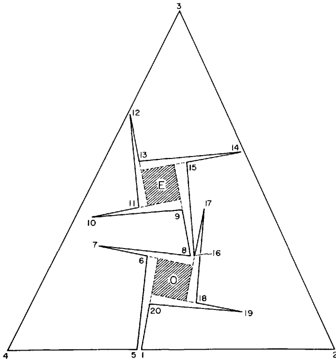
Fig. 6.2. Guards on the even vertices leave E uncovered, and guards on the odd vertices leave O uncovered.
