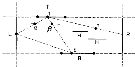
Fig. 2.6. If T and B are neighbors, then \square(L \# B, R \# T) is empty.
