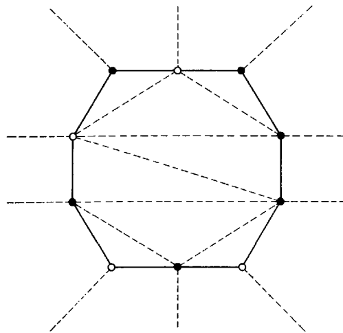
Fig. 6.16. A 10-node graph that requires 6 combinatorial guards (solid dots) for domination.
