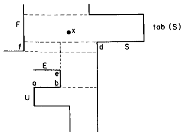
Fig. 2.17. U is the highest up tab, and S its step edge.
