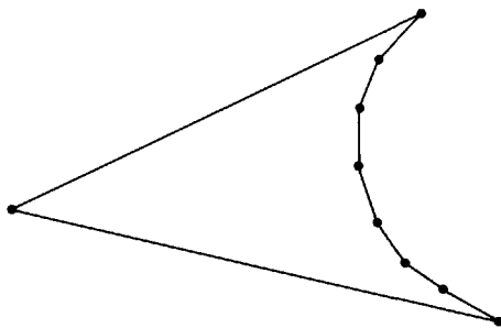
Fig. 1.26. Of a polygon’s n vertices, as many as n - 3 may be reflex.
