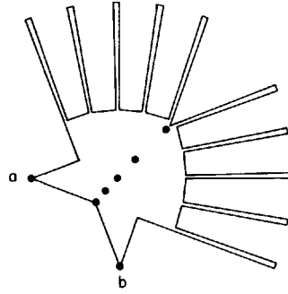
Fig. 9.1. A polygon that may be covered with 2 stars with kernels at a and b , but that requires 5 stars in a partition, with kernels at the indicated points.
