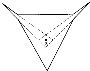
Fig. 1.5. Point guards are more powerful than vertex guards.
