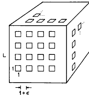
Fig. 10.2. Exterior view of Seidel's polyhedron showing array of dents.
