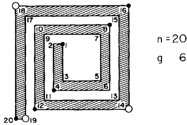
Fig. 6.4. An orthogonal spiral requires \lceil n/4 \rceil + 1 vertex guards (solid) to cover the exterior.
