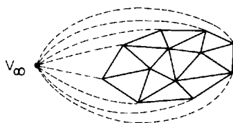
Fig. 6.13. Connecting every hull vertex to v_\infty leads to \lfloor 2n/3 \rfloor guards.
