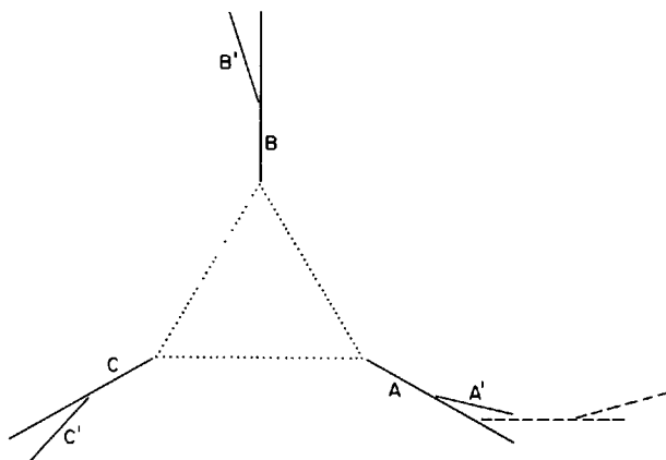
Fig. 10.9. Additional segments added to the pattern of Fig. 10.8, which is nested within the dotted triangle.
