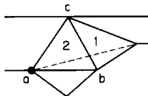
Fig. 5.17. Flipping a 21 c-pair leads to the case considered in Fig. 5.6.
