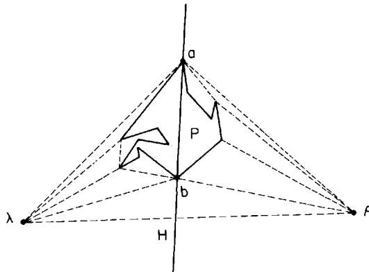
Fig. 6.8. Domination of this graph implies coverage of the exterior of the polygon.
