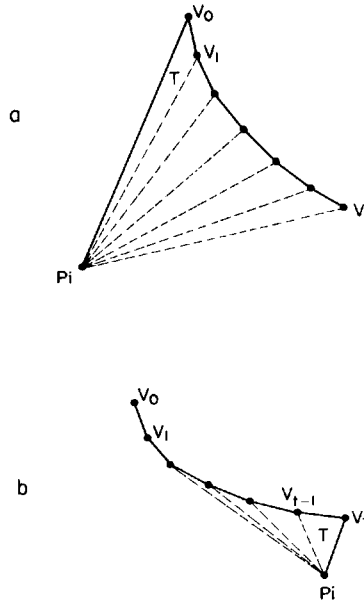
Fig. 1.21. Triangulation algorithm cases: p_i is adjacent to the stack bottom (a) or to the stack top (b).
