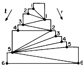
Fig. 2.20. Quadrilateralization of a pyramid by list merging.
