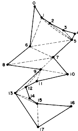
Fig. 1.22. Triangulation algorithm example.
