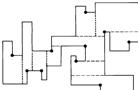
Fig. 2.61. Guards positioned in the polygon of Fig. 2.55. The dashed lines are the horizontal cuts made in step (4) of the algorithm, and the dotted lines are the vertical cuts implicit in step (5). Here r = 19 , and \lfloor r/2 \rfloor + 1 = 10 guards are used.
