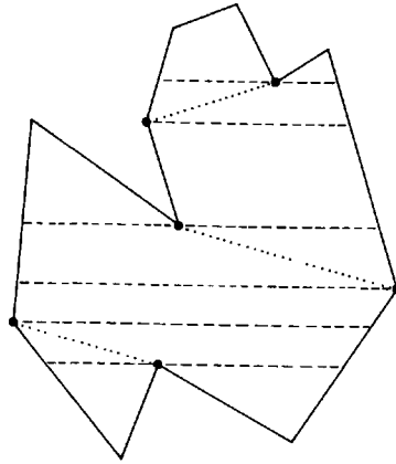
Fig. 1.23. A trapezoidization (dashed lines) leads to a monotone partitioning with the addition of diagonals to “internal” vertices (dotted).
