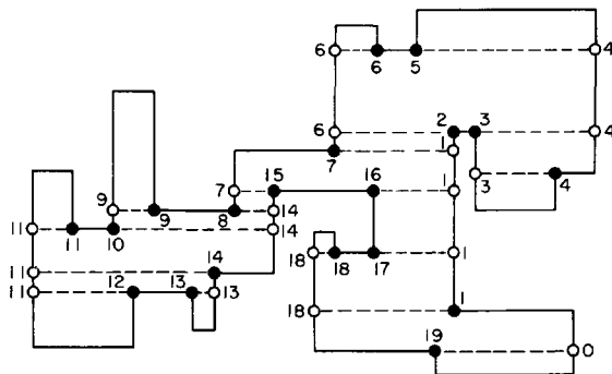
Fig. 2.55. Labels on reflex (solid dots) and artificial vertices (open circles) are generated in a counterclockwise scan of the boundary, incrementing the label counter at each reflex vertex.
