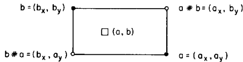
Fig. 2.5. Definition of the “ \# ” and “ \square ” symbols.
