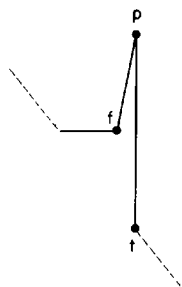
Fig. 9.10. A literal pattern. The distinguished point p is visible only to t and f .
