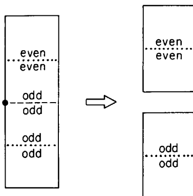
Fig. 2.58. If the total number of reflex vertices is odd, then partitioning at an odd-cut does not affect the parity of other cuts.
