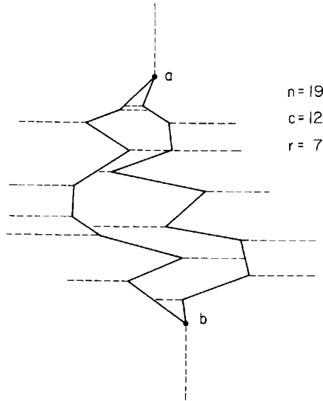
Fig. 6.20. A convex partitioning of the plane induced by a monotone polygon with 12 convex and 7 reflex vertices.
