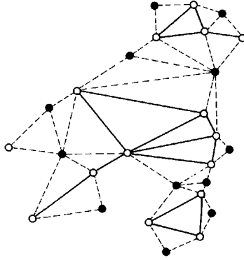
Fig. 6.14. The dashed edges are incident on a guarded vertex (solid dots).
