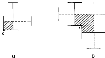
Fig. 7.21. Regions between adjacent edge nodes must be bound by 2(a) or 4(b) chords.
