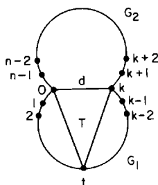
Fig. 1.9. Diagonal d cuts off k vertices in G_1 .
