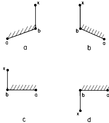
Fig. 2.40. b always has an upper neighbor; the shading indicates the interior of the polygon.
