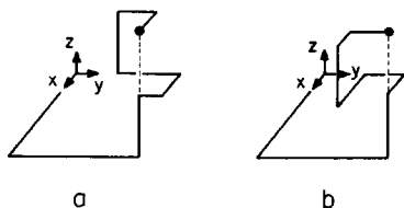
Fig. 9.17. Bending a path to avoid overlap on the -z ray, to enter along the -x ray (a) or the -y ray (b).
