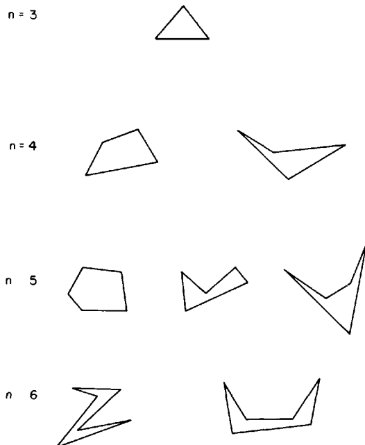
Fig. 1.1. Polygons with 5 or fewer vertices can be covered by a single guard, but some 6-vertex polygons require two guards.
