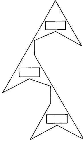
Fig. 5.4. A polygon of 24 vertices with 3 holes that requires 9 guards.
