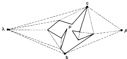
Fig. 6.10. If the number of hull vertices is even, this graph is 3-colorable.
