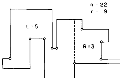
Fig. 2.45. A cut partitions a polygon into two pieces of L and R reflex vertices; since the cut resolves one reflex vertex, r = L + R + 1 .
