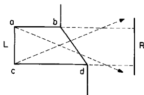
Fig. 2.7. A tab (ab, cd) forces the inclusion of quadrilateral abcd .
