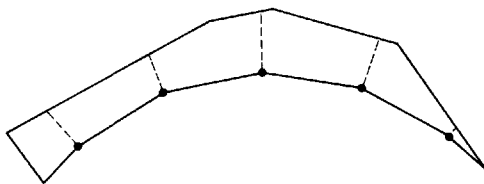
Fig. 4.8. A partition of a spiral polygon into r + 1 convex pieces.
