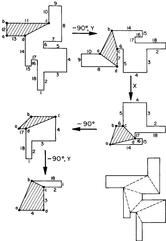
Fig. 2.37. Quadrilateralization by repeated deletion of a removable quadrilateral. The notation “ -90^\circ, Y ” means that the figure is rotated 90^\circ clockwise and then reflected in the Y -axis; the remaining arrow labels may be interpreted similarly.
