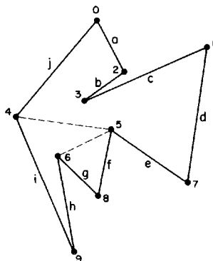
Fig. 1.19. Monotone partitioning example: diagonals (5, 4) and (6, 5) partition the polygon into monotone pieces.
