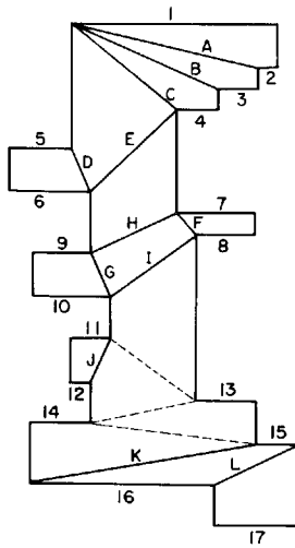
Fig. 2.23. A partition produced by the monotone quadrilateralization algorithm.
