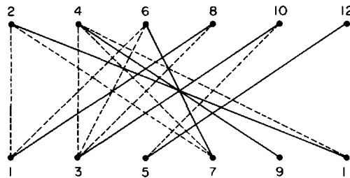
Fig. 9.15. The intersection graph for the grid in Fig. 9.14. The 6 guards are shown as solid lines.
