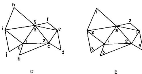
Fig. 1.6. Three-coloring of a triangulation graph starting from acg .
