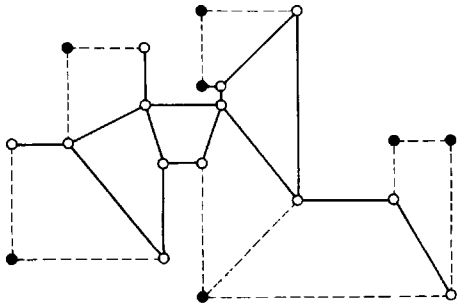
Fig. 6.15. The dashed edges are adjacent to a guard as in Fig. 6.14.
