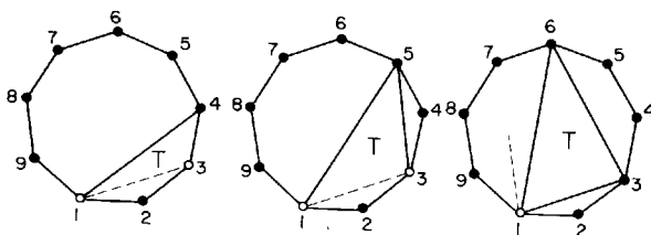
Fig. 3.5. A enneagon can be dominated by two diagonal guards, with one of their ends at node 1.
