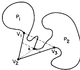
Fig. 1.13. The line segment xv_2 is an internal diagonal.
