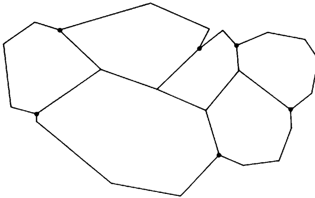
Fig. 1.28. An optimal convex partition may require interactions between the cuts resolving several reflex vertices.
