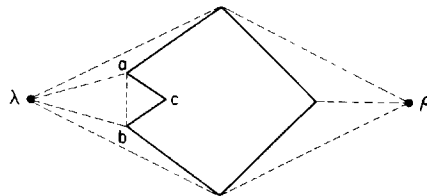
Fig. 6.9. A graph that requires 3 combinatorial guards for dominance, but only 2 point guards are needed for coverage of the exterior.
