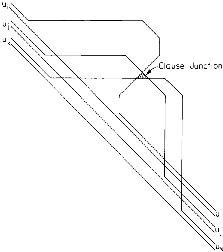
Fig. 9.9. Arrangement of variable loops and a clause junction.
