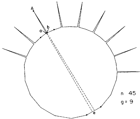
Fig. 4.4. A star polygon requiring \lfloor n/5 \rfloor edge guards.
