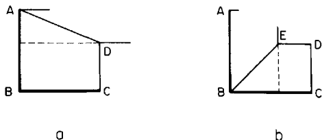
Fig. 3.26. If ABCD has degree 1 and AB and BC are guarded, one quadrilateral may be removed.
