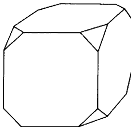
Fig. 10.5. The result of truncating a cube at every vertex.
