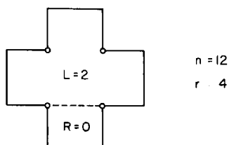
Fig. 2.46. A polygon that does not admit an odd-cut, but that permits a single cut to resolve two reflex vertices.
