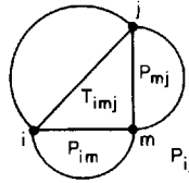
Fig. 9.18. The subpolygon P_{ij} and associated regions.
