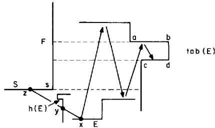
Fig. 2.16. There must exist a bottom edge h(E) in the illustrated situation.
