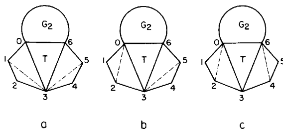
Fig. 1.11. G_1 is a heptagon.
