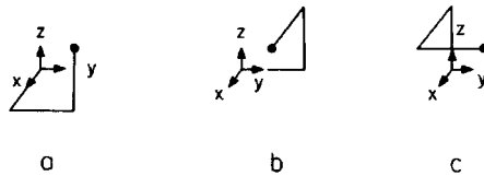
Fig. 9.16. Three paths from v_i (the origin) to v_j .
