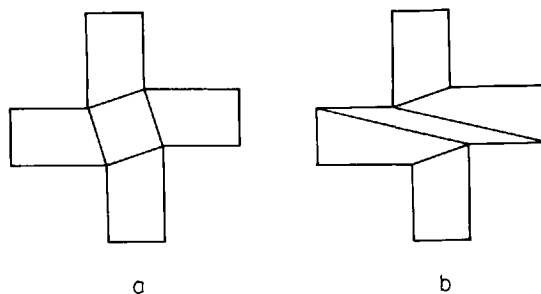
Fig. 2.2. Quadrilateralization is not unique.
