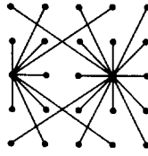
Fig. 10.12. A 5 \times 5 lattice in which two points can see all the other points.
