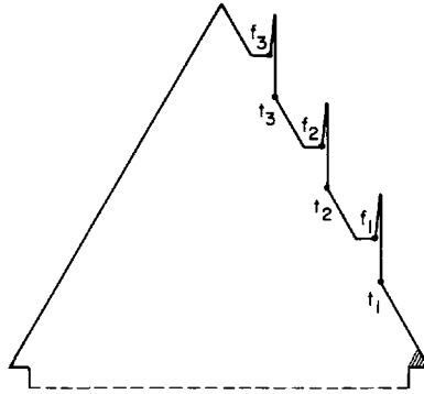
Fig. 9.11. A clause junction. The shaded triangle can be seen only by t_i , i = 1, 2, 3 .
