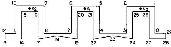
Fig. 1.3. Guards on every third vertex will not cover one of the points x_0 , x_1 , or x_2 .
