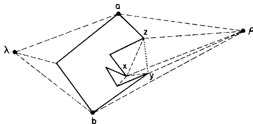
Fig. 6.11. If the number of hull vertices is odd, one vertex x within the hull is connected to p to make a 3-colorable graph.
