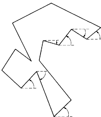
Fig. 1.25. A polygon with sinuosity 1: there are no two successive clockwise transitions across the horizontal.
