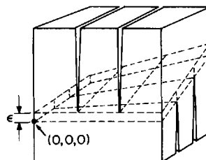
Fig. 10.4. Any convex partition of Chazelle's polyhedron requires a quadratic number of pieces.
