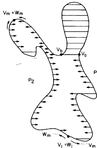
Fig. 1.24. Stitching together trapezoids from separate chains to form a trapezoidization.
