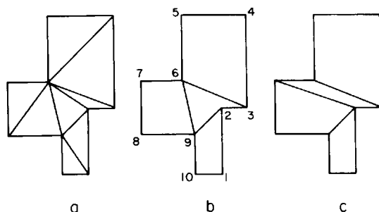
Fig. 2.1. Neither triangle pairing (a) nor ear removal (b) can lead to the unique quadrilateralization (c).
