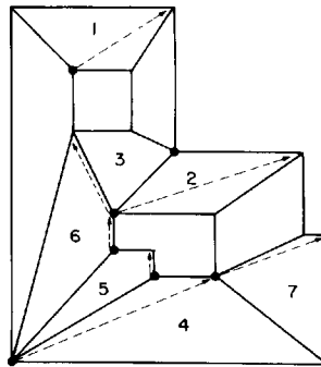
Fig. 2.43. Quadrilateralization by repeated deletion of removable quadrilaterals. The quadrilaterals are numbered in the order in which they are removed. The dashed arrows represent the upper neighbor relation.
