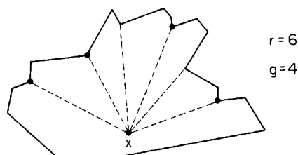
Fig. 4.3. A partition of a star made by connecting a kernel point x to every reflex vertex.
