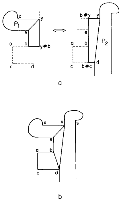
Fig. 2.11. Good tab reduction for Fig. 2.10a.
