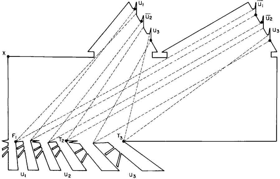
Fig. 9.13. The complete polygon for (u_1 + \bar{u}_2 + u_3) \cdot (\bar{u}_1 + \bar{u}_2 + u_3) .
