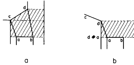
Fig. 2.27. The diagonals chosen by the algorithm pass through empty (shaded) regions.
