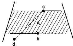
Fig. 2.41. The region A between b and its upper neighbor c .
