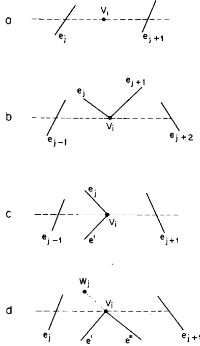
Fig. 1.18. Notation and sweep line events for monotone partitioning algorithm.
