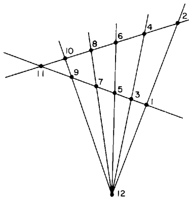
Fig. 10.11. A configuration in which no point can see more than 8 = 12/2 + 2 other points.
