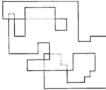
Fig. 2.4. An orthogonal polygon lying on several levels.
