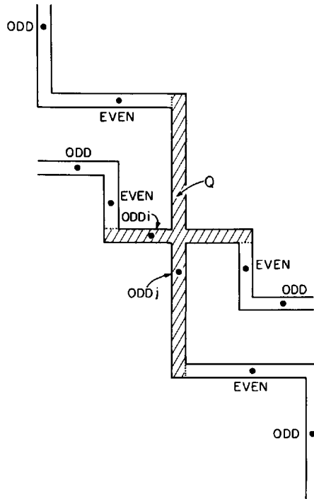
Fig. 9.6. Variable loop crossover. Star Q contains two odd distinguished points.
