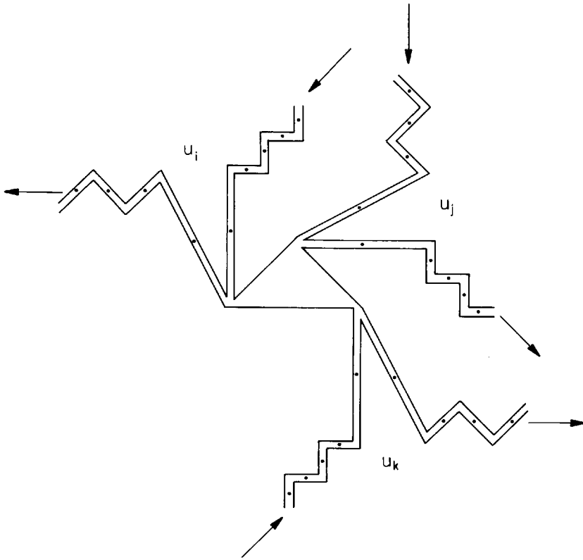
Fig. 9.8. A clause junction. The central triangle is covered free iff the corresponding clause is satisfied.
