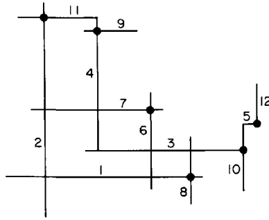
Fig. 9.14. A grid covered by 6 guards (dots).
