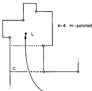
Fig. 2.50. If a leaf region L has k > 0 H-isolated vertices, then it admits an H-odd-cut.
