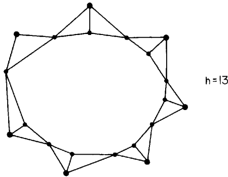
Fig. 6.12. Addition of \lceil h/2 \rceil nodes exterior to the hull leads to n/2 + h/4 guards (modulo floors and ceilings).
