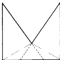
Fig. 9.2. A polygon that may be covered with 2 convex pieces if Steiner points are permitted (dashed), but requires 3 if not permitted (dotted).
